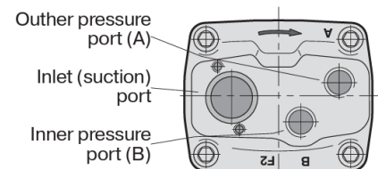
End cap for left hand rotating pump
