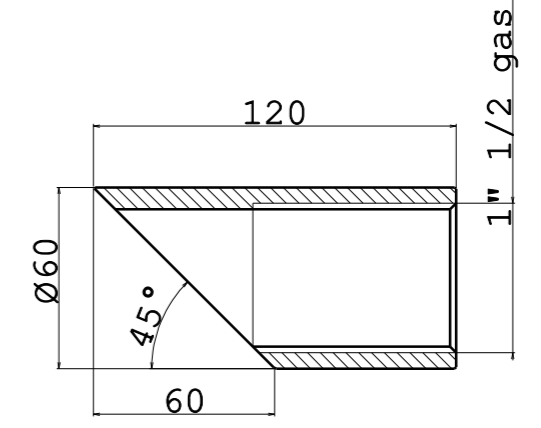
4 1"1/2 SUCTION ADAPTER
