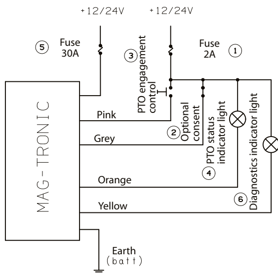
WIRING DIAGRAM
