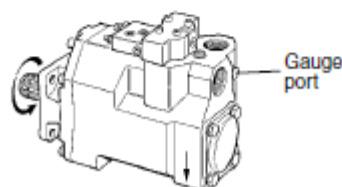
Fig. 5. Right hand rotating pump.
