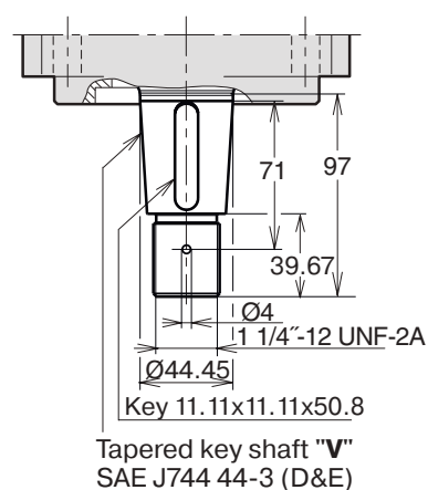
Shaft option V (F12-60)
