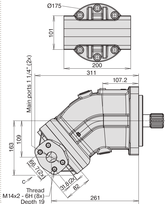
Main ports type M (Side ports)
