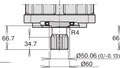
Shaft option F
