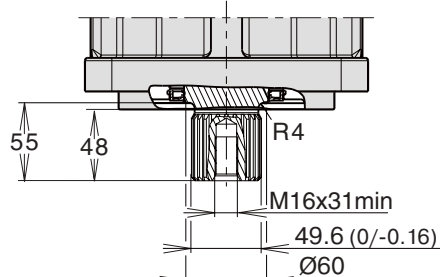
Shaft option D
