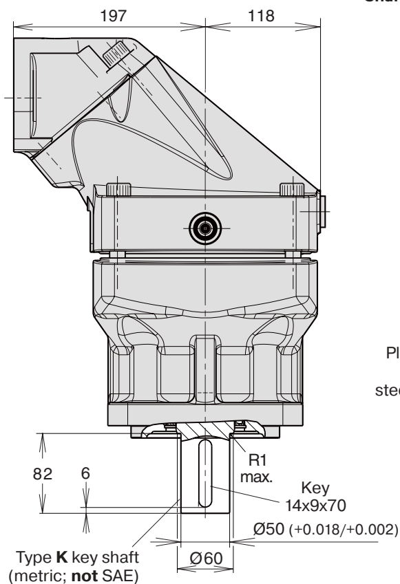
Shaft option K
